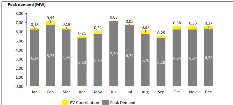
Figure 8: Monthly peak demand with and without PV generation
