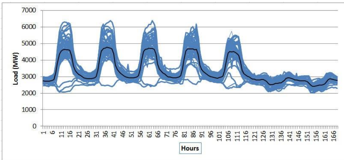
Figure 4: Weekly demand profile for the entity
